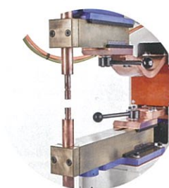
Quick set-up by the square-shaped horn.
